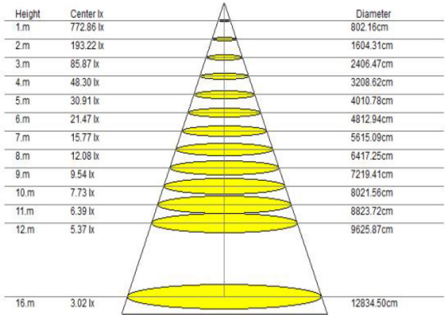
Beam Angle: 152.00° (50%Imax)
