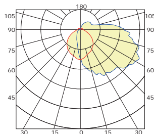
Luminous Intensity Distribution Curve
