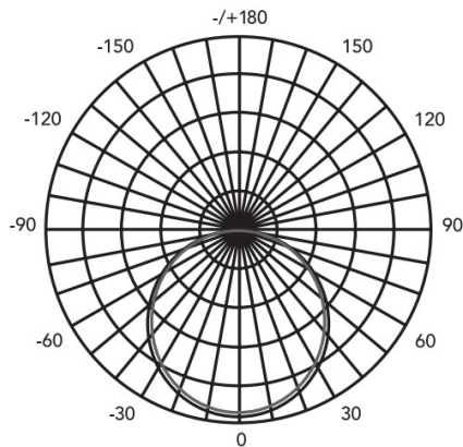
AVERAGE BEAM ANGLE (50%) : 114.3 DEG
