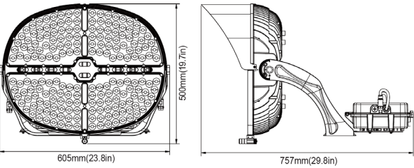
Large Size: 850W & 1200W
