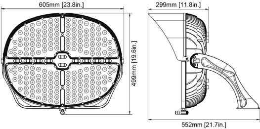
Large Size: 850W & 1200W
