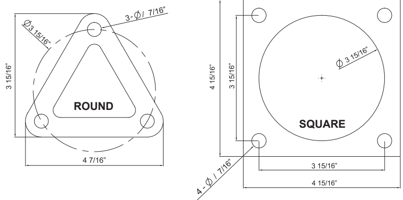
Anchor Bolt Template (Drawing not to scale)
