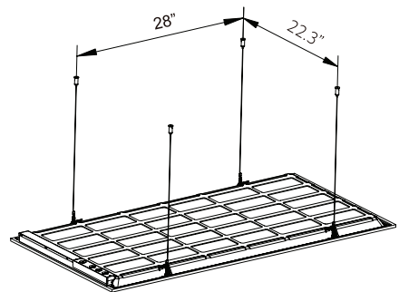
EBS-SCM-14-S 4-Cable Kit
