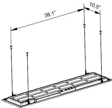
EBS-SCM-14-S 4-Cable Kit
