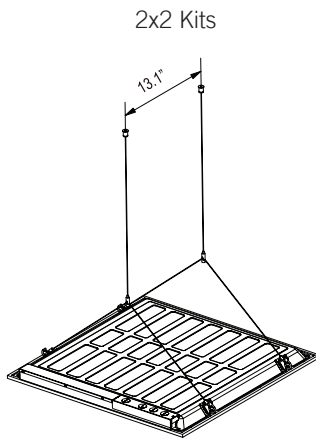
EBS-SCM-12-S 2-Cable Kit
