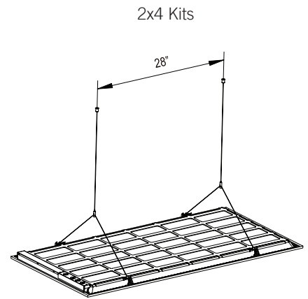
EBS-SCM-12-S 2-Cable Kit
