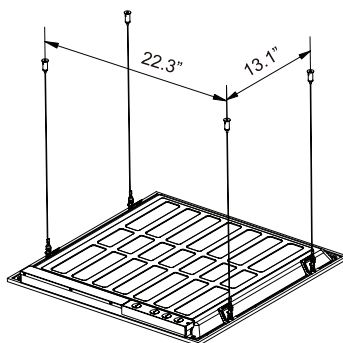
EBS-SCM-14-S 4-Cable Kit
