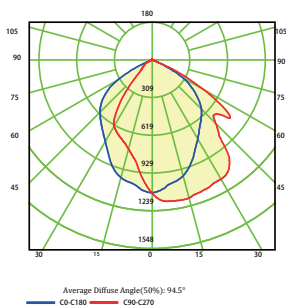
Luminous Intensity Distribution Curve 20W
