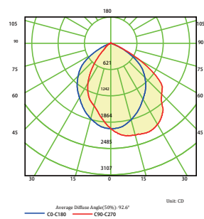
Luminous Intensity Distribution Curve 40W
